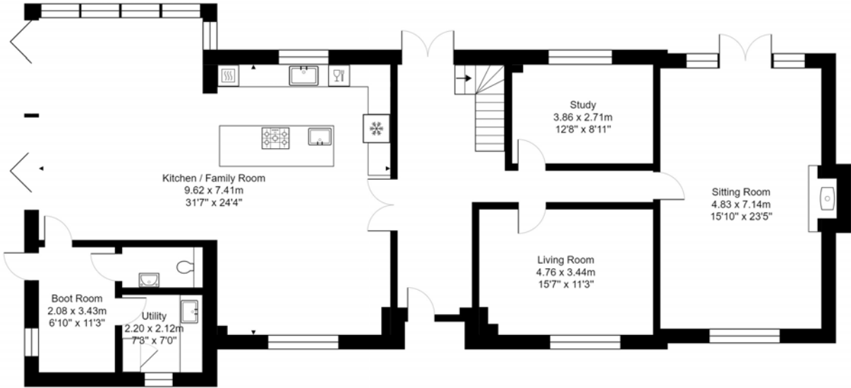
Ground Floor Area: 166.5 m² ... 1792 ft²
