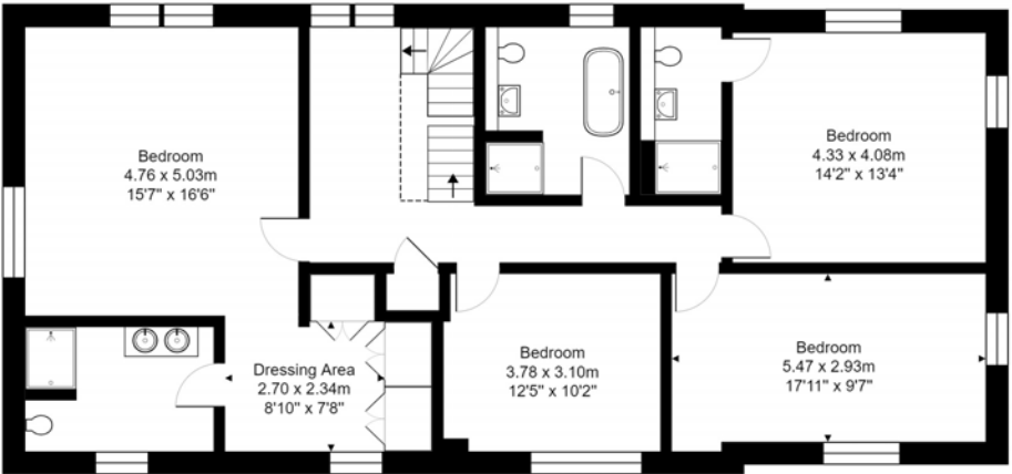
First Floor Area: 122.7 m² ... 1321 ft²
